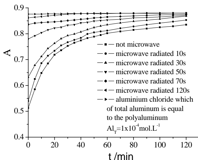
Fig. 1 The comparison of the alteration of A vs. time curve when polyaluminium solutions was radiated different time by microwave ( \bar{n}=2.0 , Al_T = 1 \times 10^{-4} \text{ mol L}^{-1} )
